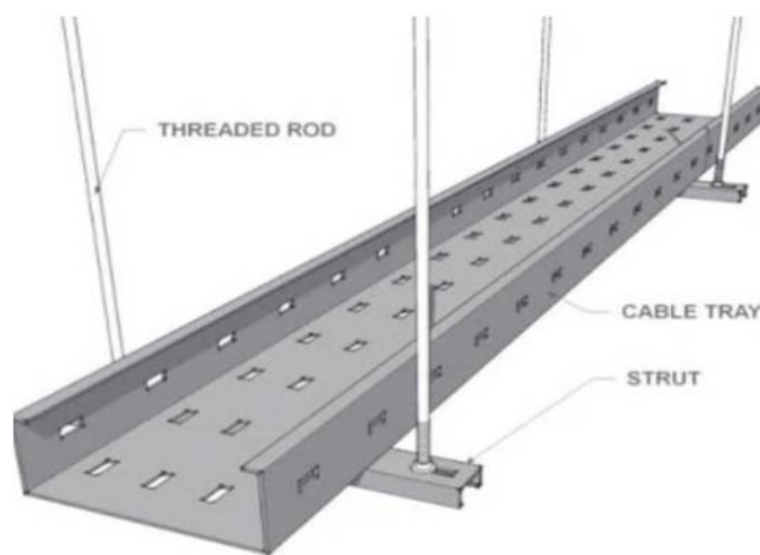
Gi Perforated Cable Tray & Tie Rod
